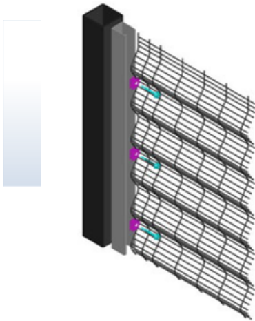
Typical Corromesh® Safety Channel Side Fixing Detail
