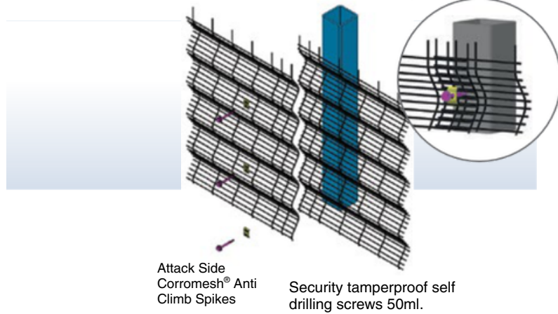
Typical Corromesh® Overlap Fixing Detail Security Washer
